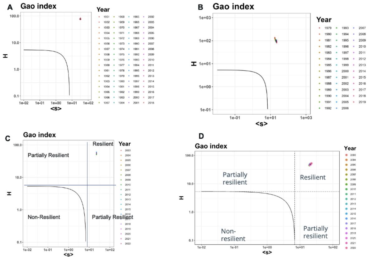
Figure 2. Preliminary Resilience (Gao Index) estimations for the (A) WCPO Warm Pool, (B) Tropical Eastern Pacific Ocean, (C) Tropical Atlantic Ocean, and (D) Tropical Indian Ocean.
