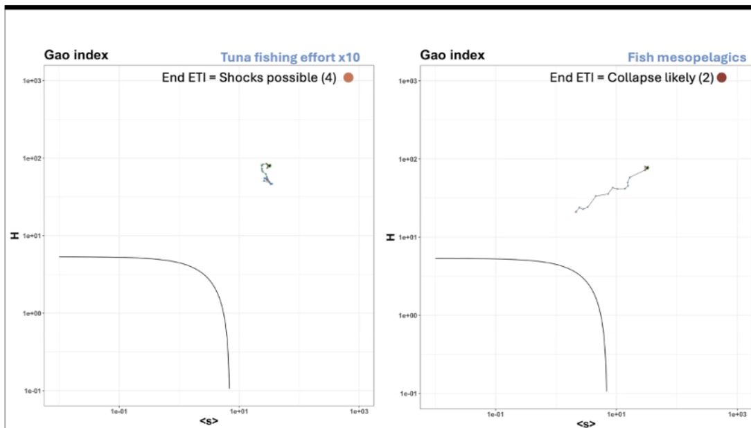
Figure 3. Resilience (Gao Index) estimations for the WCPO Warm Pool when (left) tuna fishing effort is increased by 10 and (right) mesopelagic fishes are caught unsustainably.
