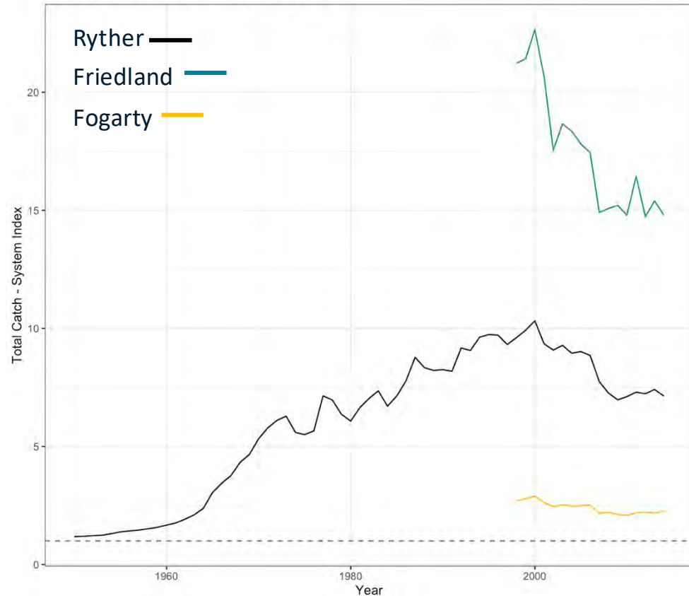
Total Catch Gulf of Thailand (1950-2015)
